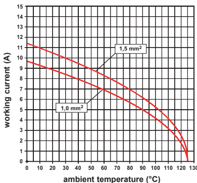
CX 12 D, 12 poles connector inserts Maximum current load derating diagram
