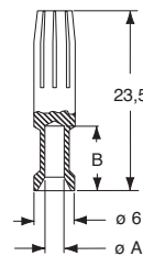
CXF and CXM contacts
