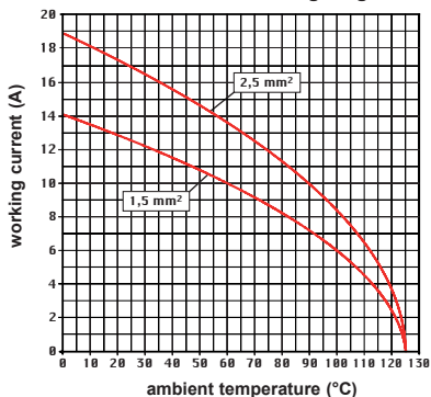
CX 05 SH, 5 power poles connector inserts Maximum current load derating diagram
