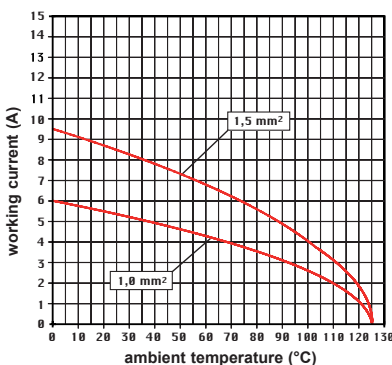
CX 17 poles connector inserts Maximum current load derating diagram
