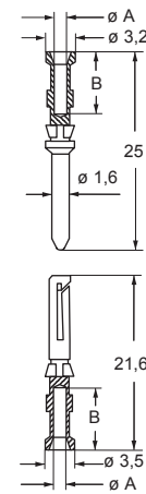
RDF2D and RDM2D contacts
