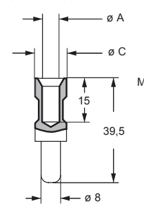
CGF and CGM
